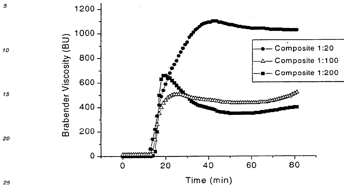
Graph 2. xanthan:waxy corn starch composite heat treated at 120C for 4hours.
